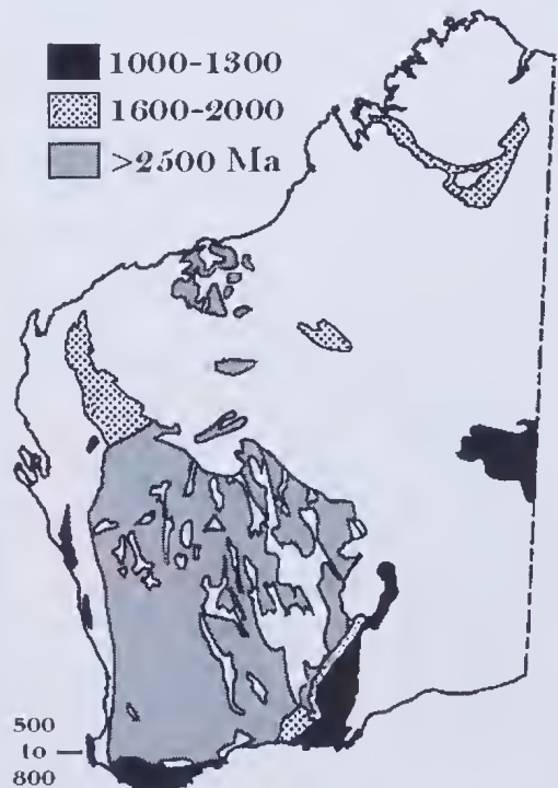
Figure 2. Approximate ages of formation of the main granite outcrops in Western Australia (modified from Myers 1997).
